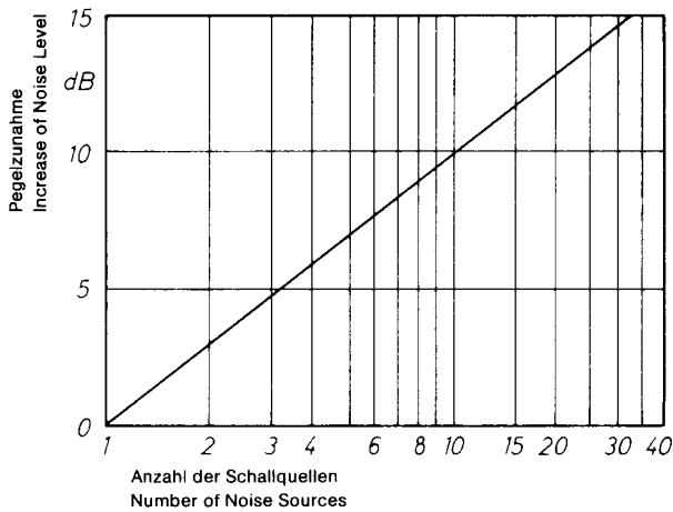
Fig. 13 Addition mehrerer Schallquellen gleichen Pegels Addition of several noise sources of equal level
